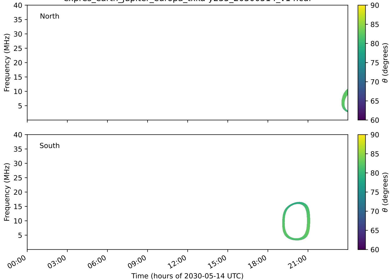
expres_earth_jupiter_europa_txka-y235_20300514_v14.cdf
