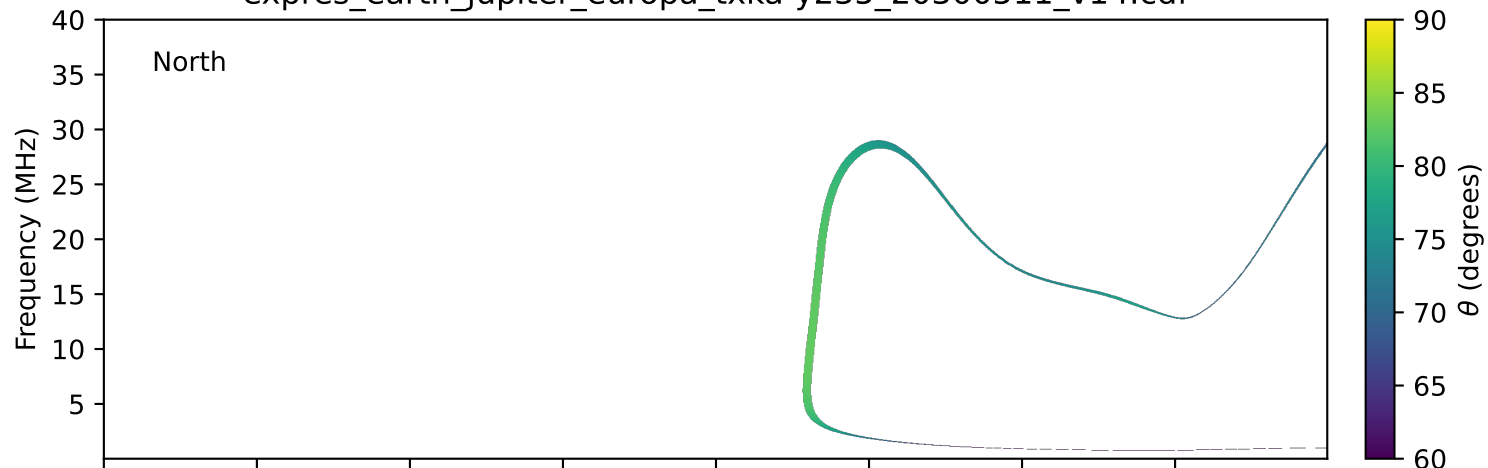
expres_earth_jupiter_europa_txka-y235_20300511_v14.cdf
