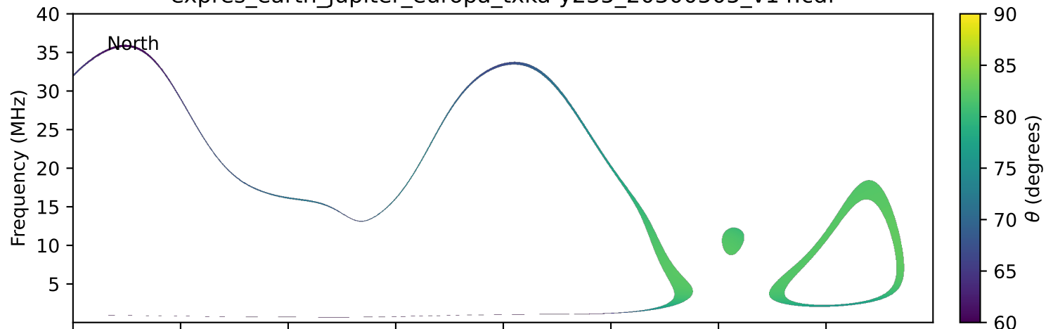
expres_earth_jupiter_europa_txka-y235_20300505_v14.cdf
