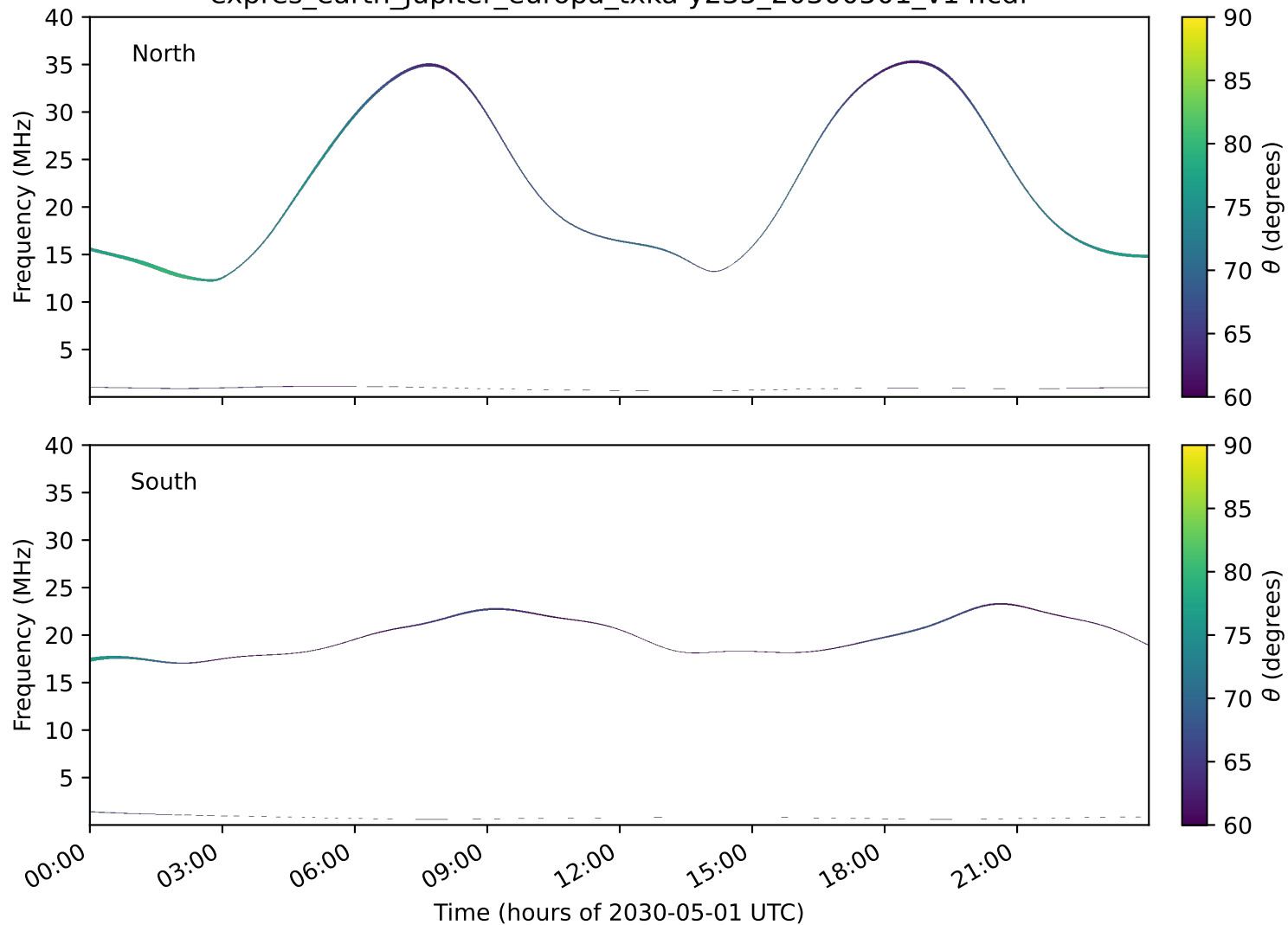
expres_earth_jupiter_europa_txka-y235_20300501_v14.cdf
