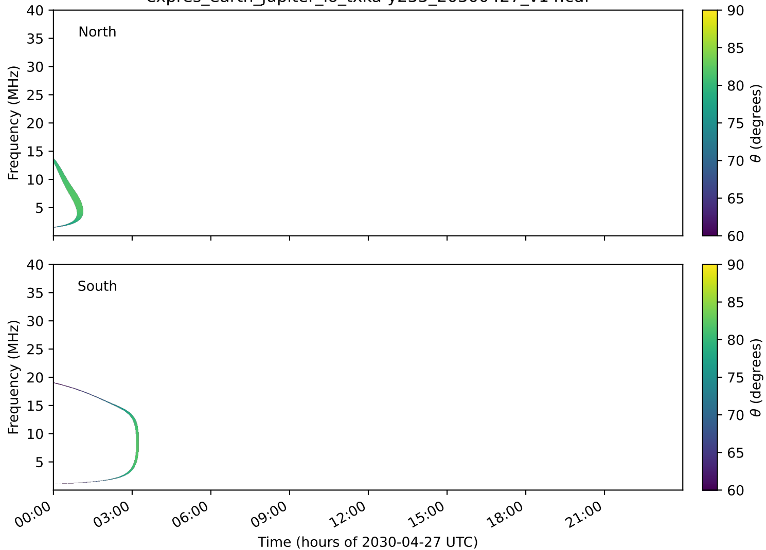
expres_earth_jupiter_io_txka-y235_20300427_v14.cdf
