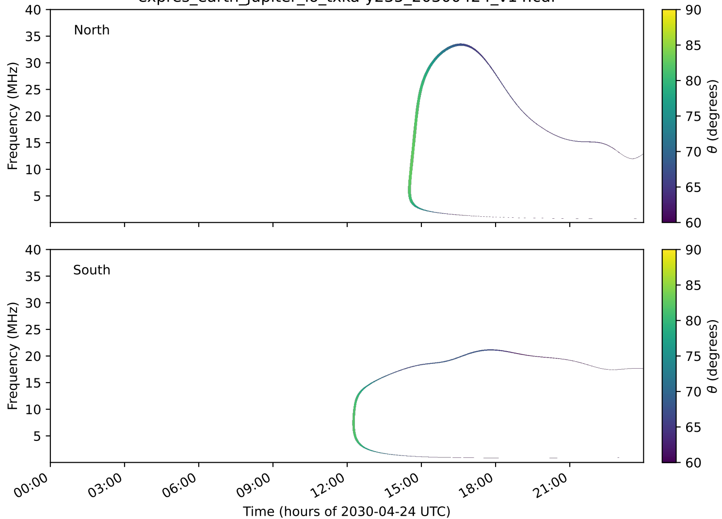
expres_earth_jupiter_io_txka-y235_20300424_v14.cdf
