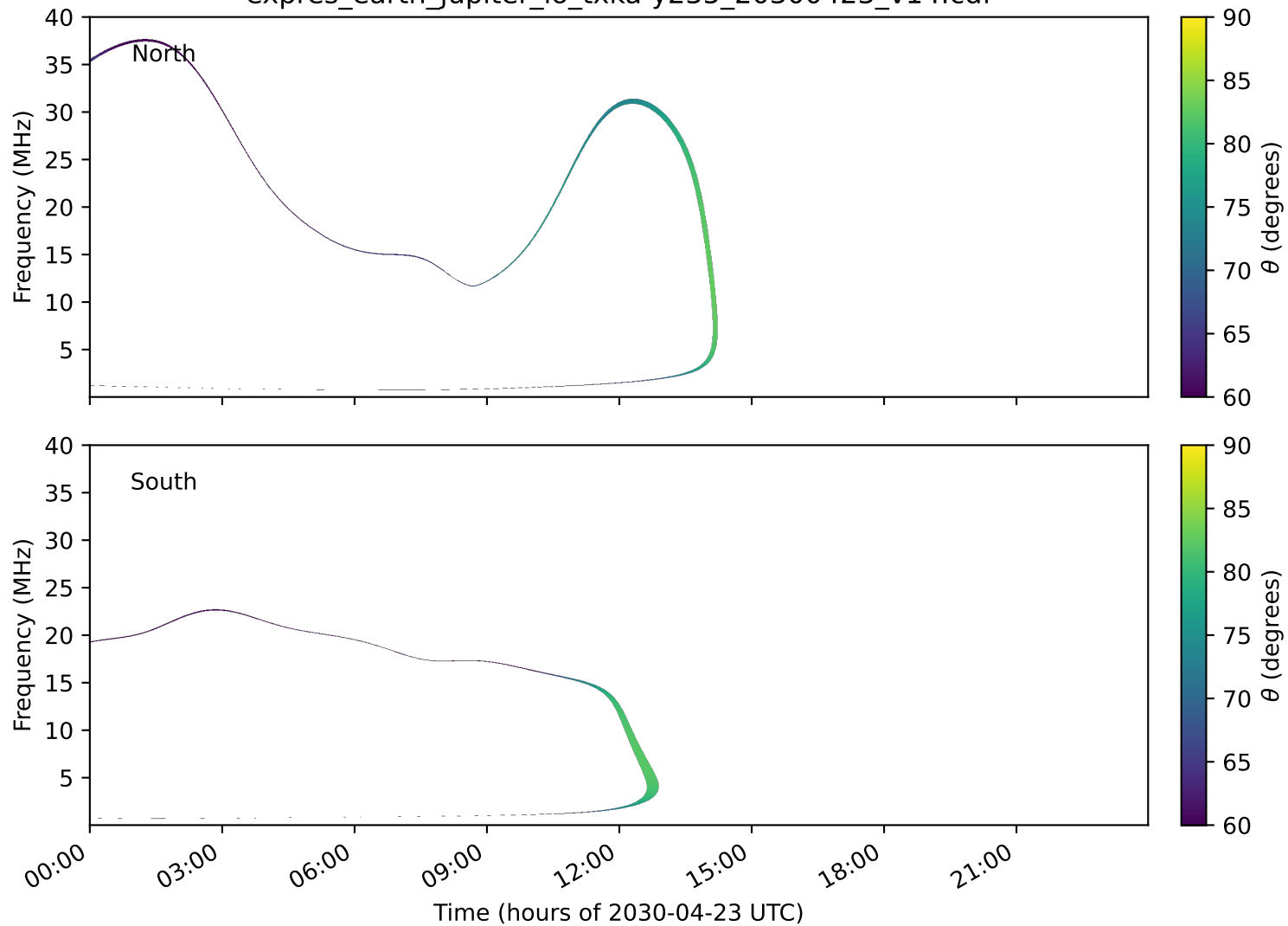
expres_earth_jupiter_io_txka-y235_20300423_v14.cdf
