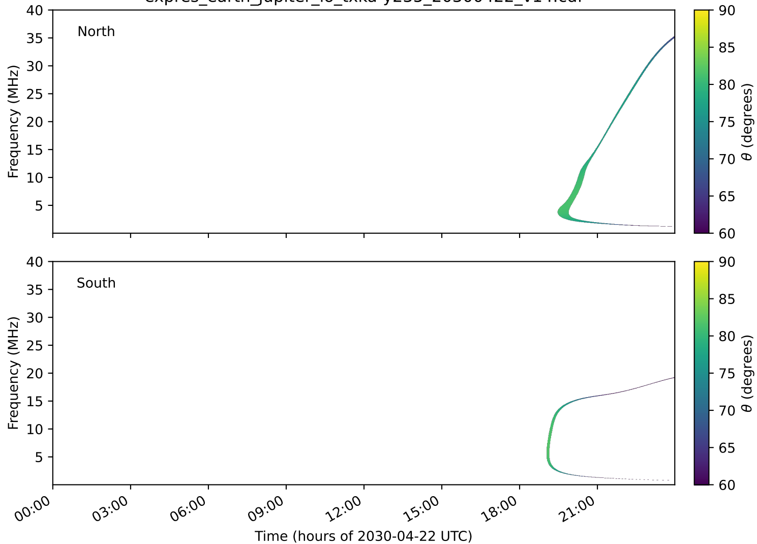
expres_earth_jupiter_io_txka-y235_20300422_v14.cdf
