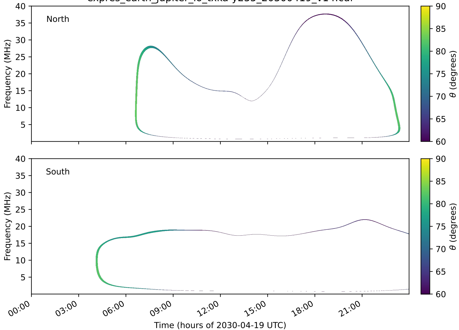
expres_earth_jupiter_io_txka-y235_20300419_v14.cdf
