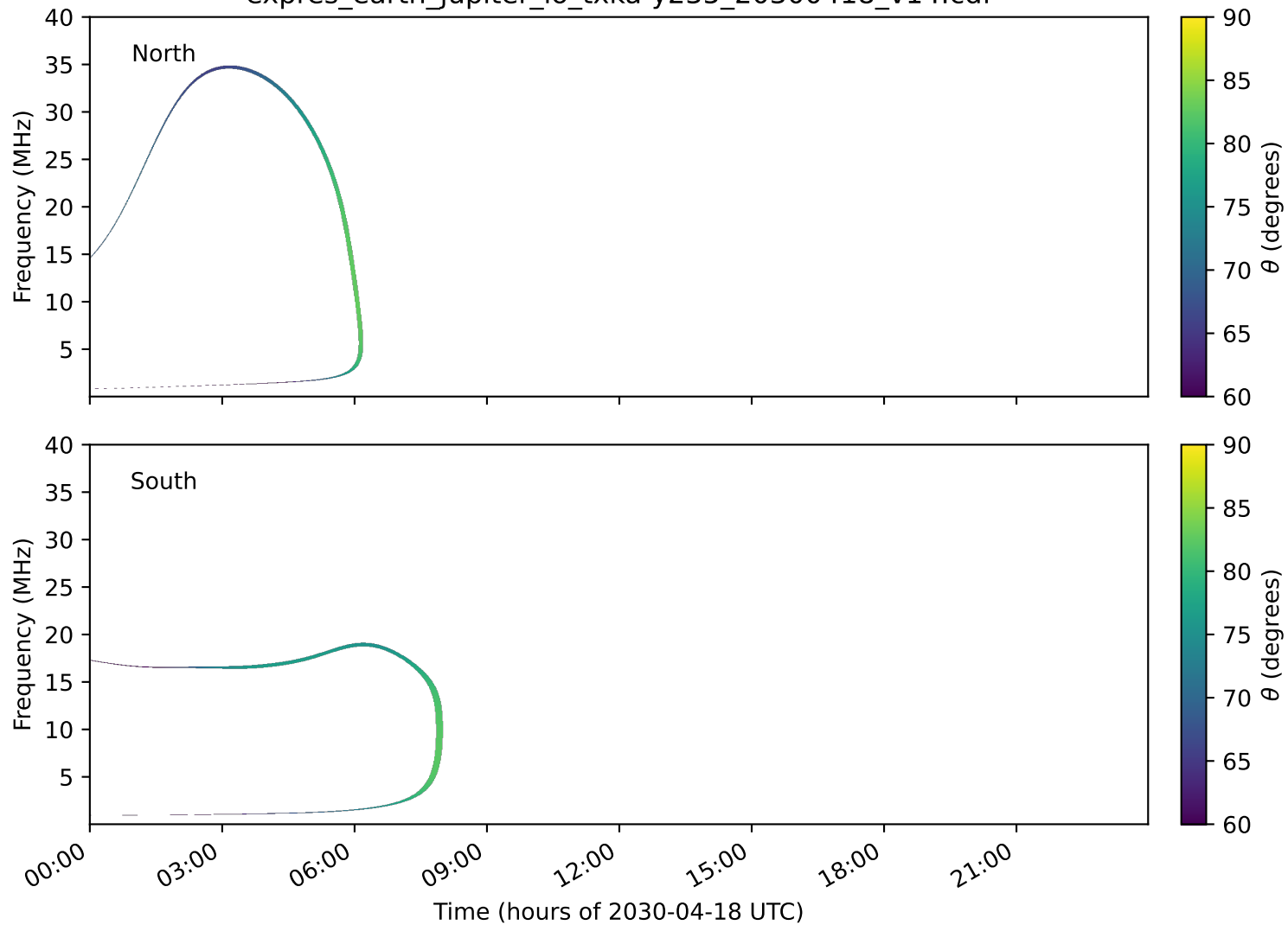
expres_earth_jupiter_io_txka-y235_20300418_v14.cdf
