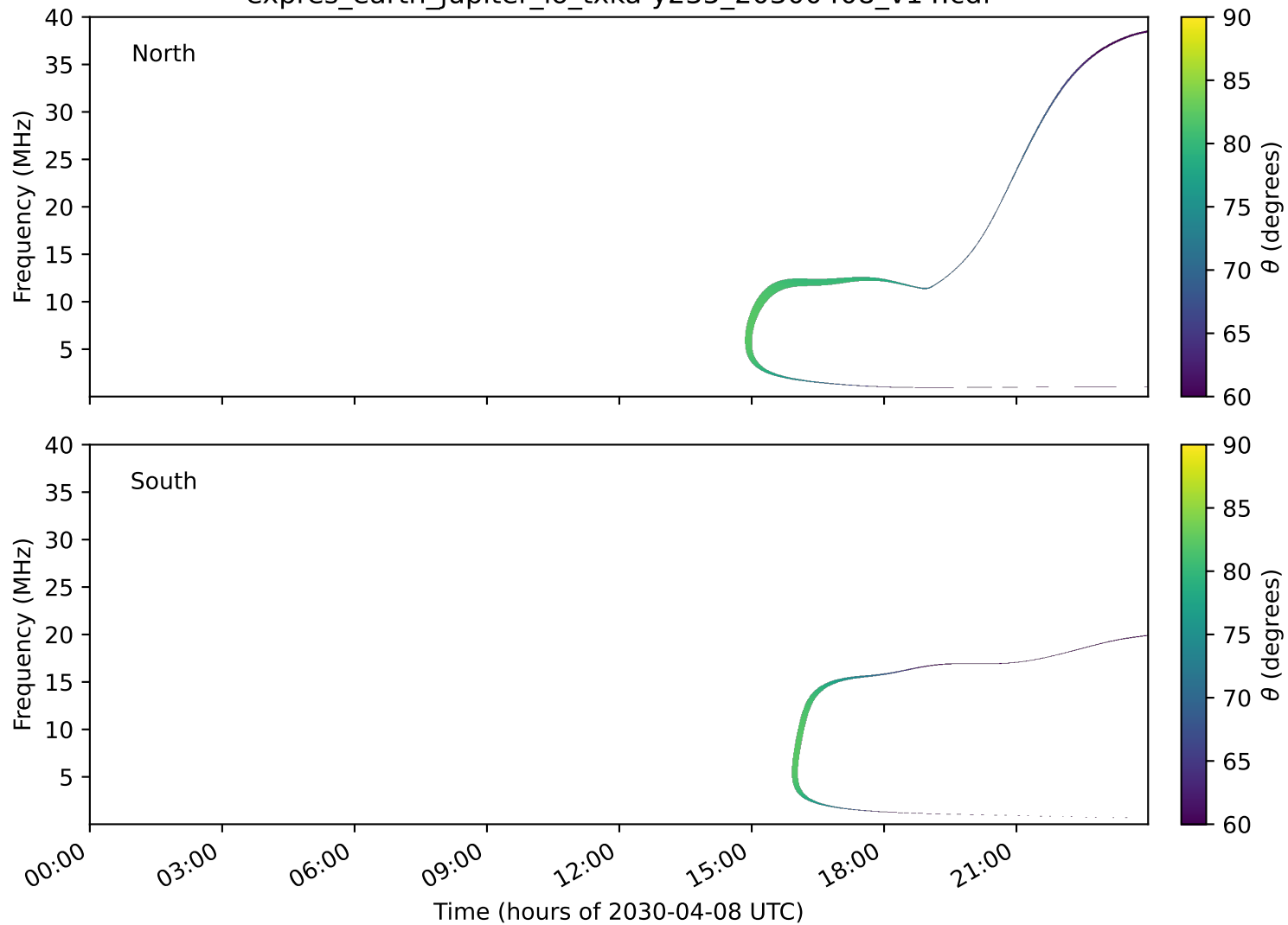
expres_earth_jupiter_io_txka-y235_20300408_v14.cdf
