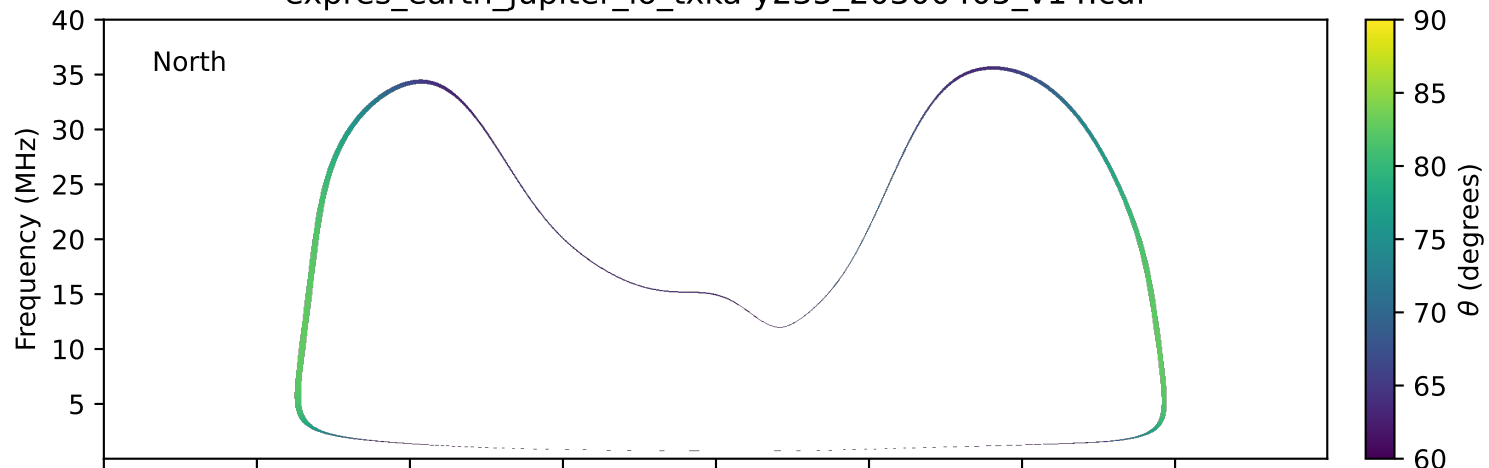
expres_earth_jupiter_io_txka-y235_20300405_v14.cdf
