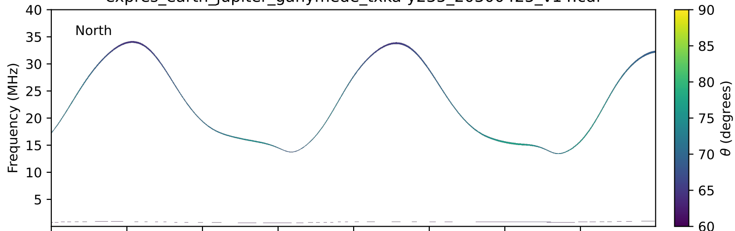
expres_earth_jupiter_ganymede_txka-y235_20300425_v14.cdf
