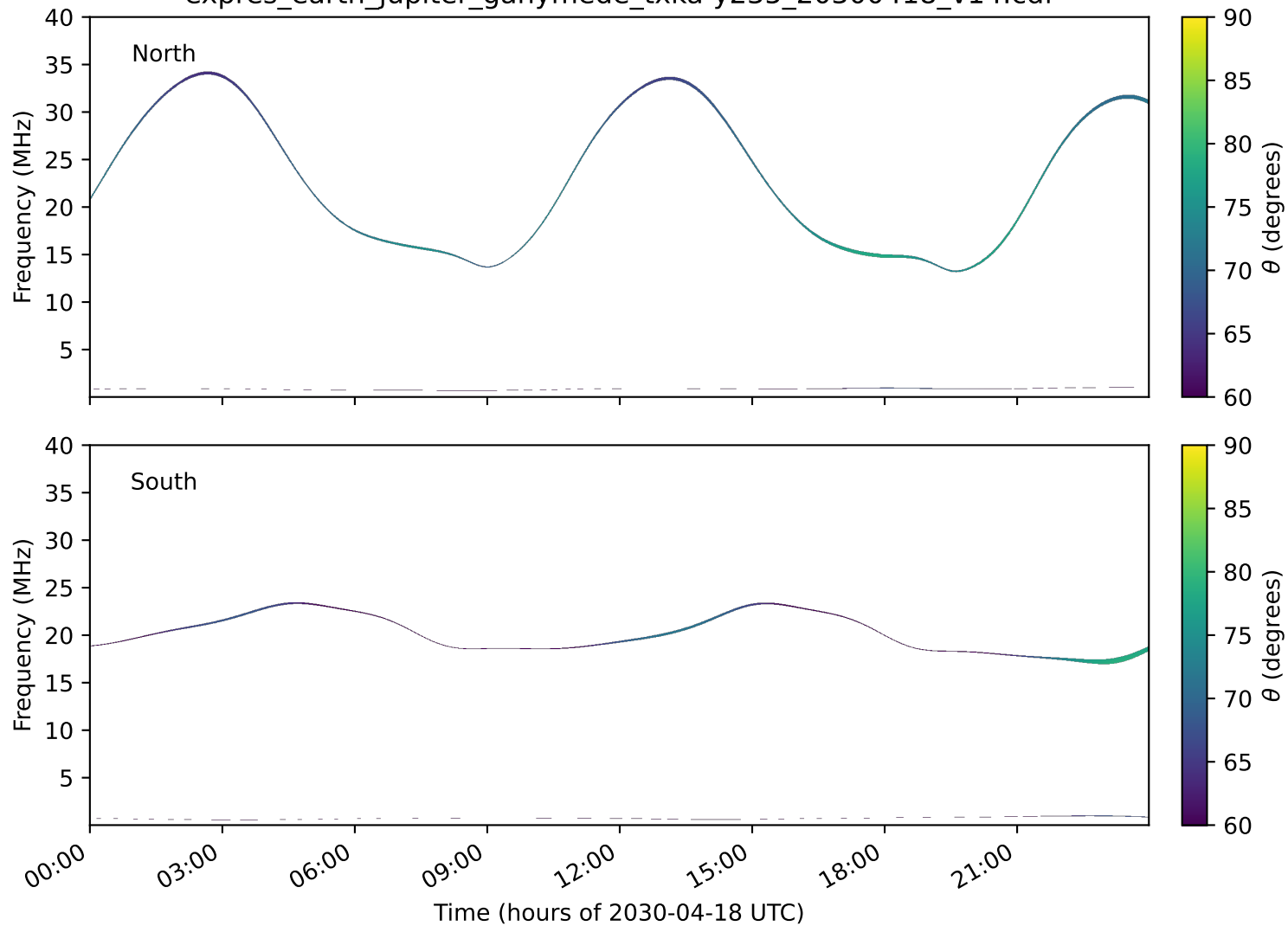
expres_earth_jupiter_ganymede_txka-y235_20300418_v14.cdf
