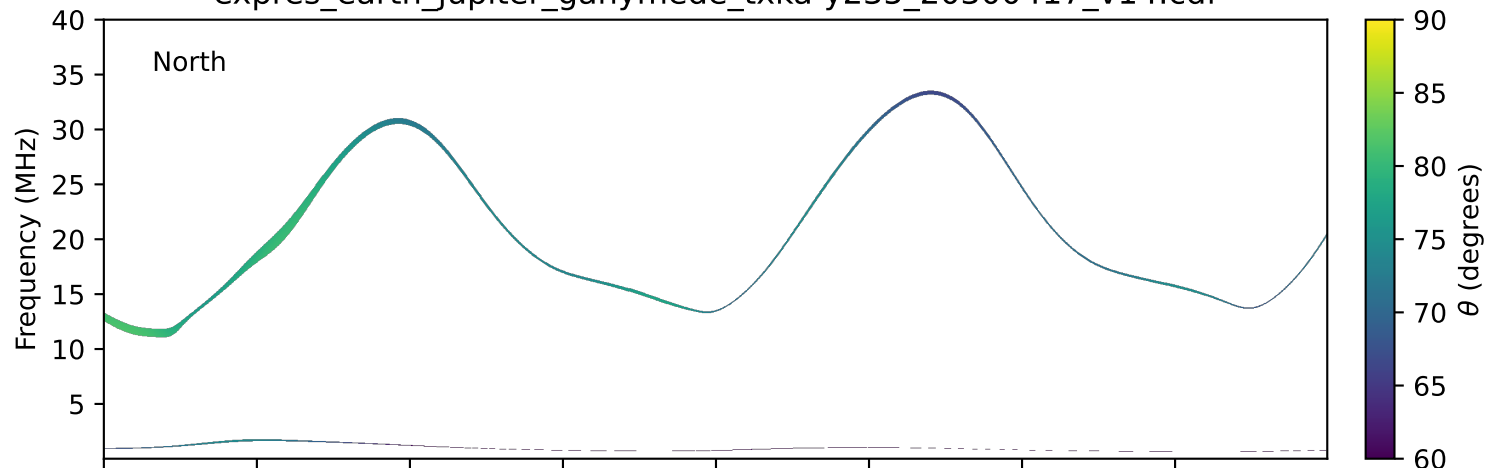
expres_earth_jupiter_ganymede_txka-y235_20300417_v14.cdf
