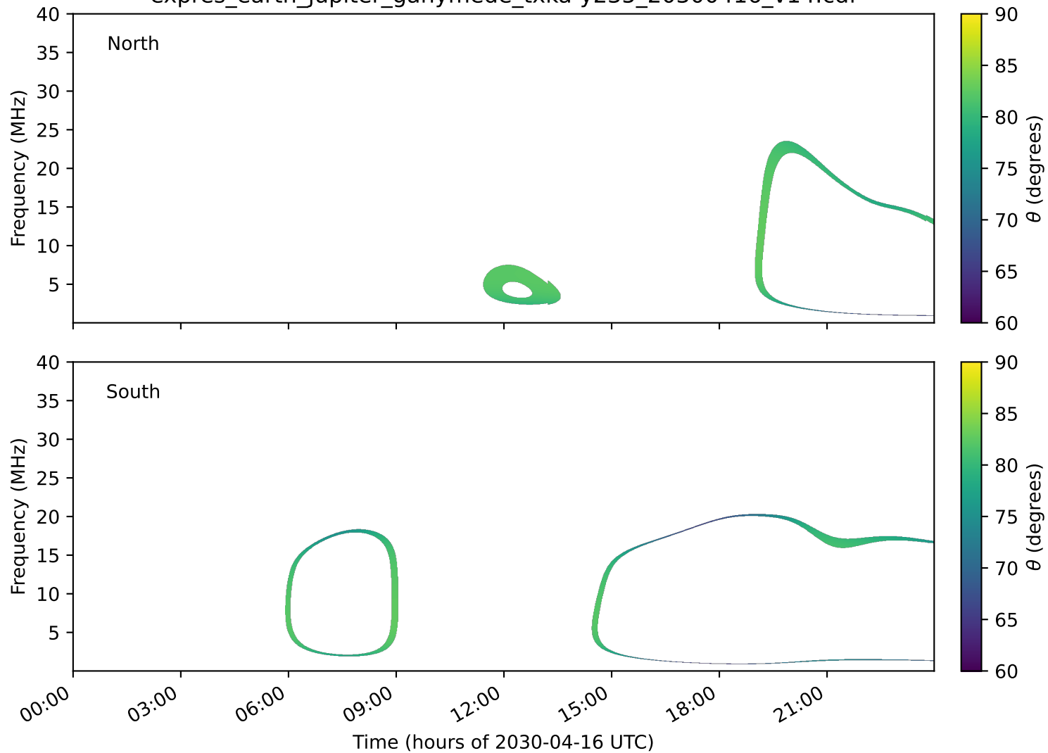
expres_earth_jupiter_ganymede_txka-y235_20300416_v14.cdf
