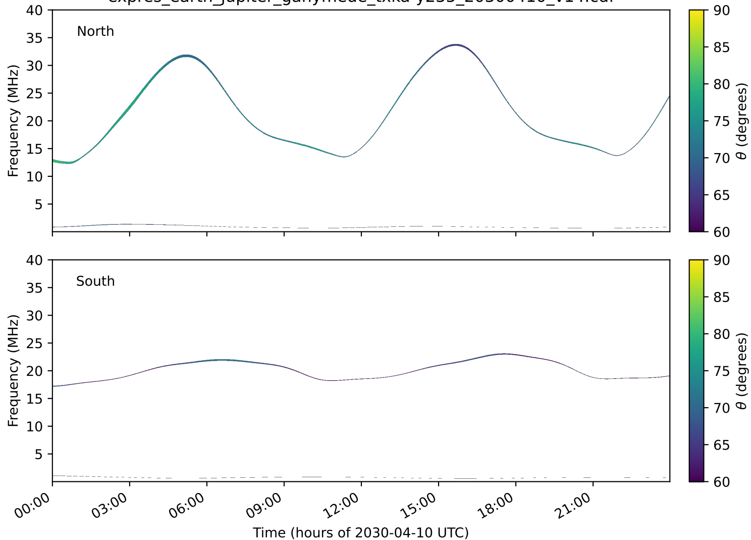
expres_earth_jupiter_ganymede_txka-y235_20300410_v14.cdf
