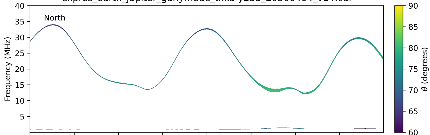
expres_earth_jupiter_ganymede_txka-y235_20300404_v14.cdf
