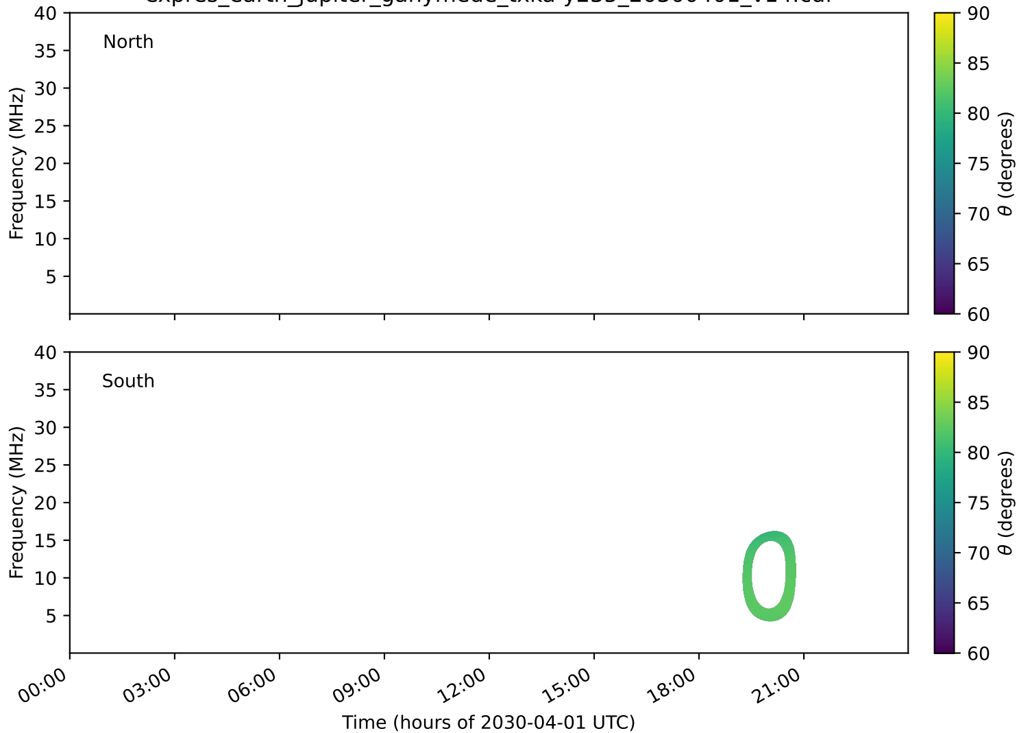
expres_earth_jupiter_ganymede_txka-y235_20300401_v14.cdf
