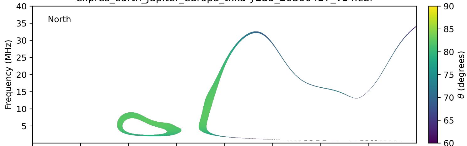
expres_earth_jupiter_europa_txka-y235_20300427_v14.cdf
