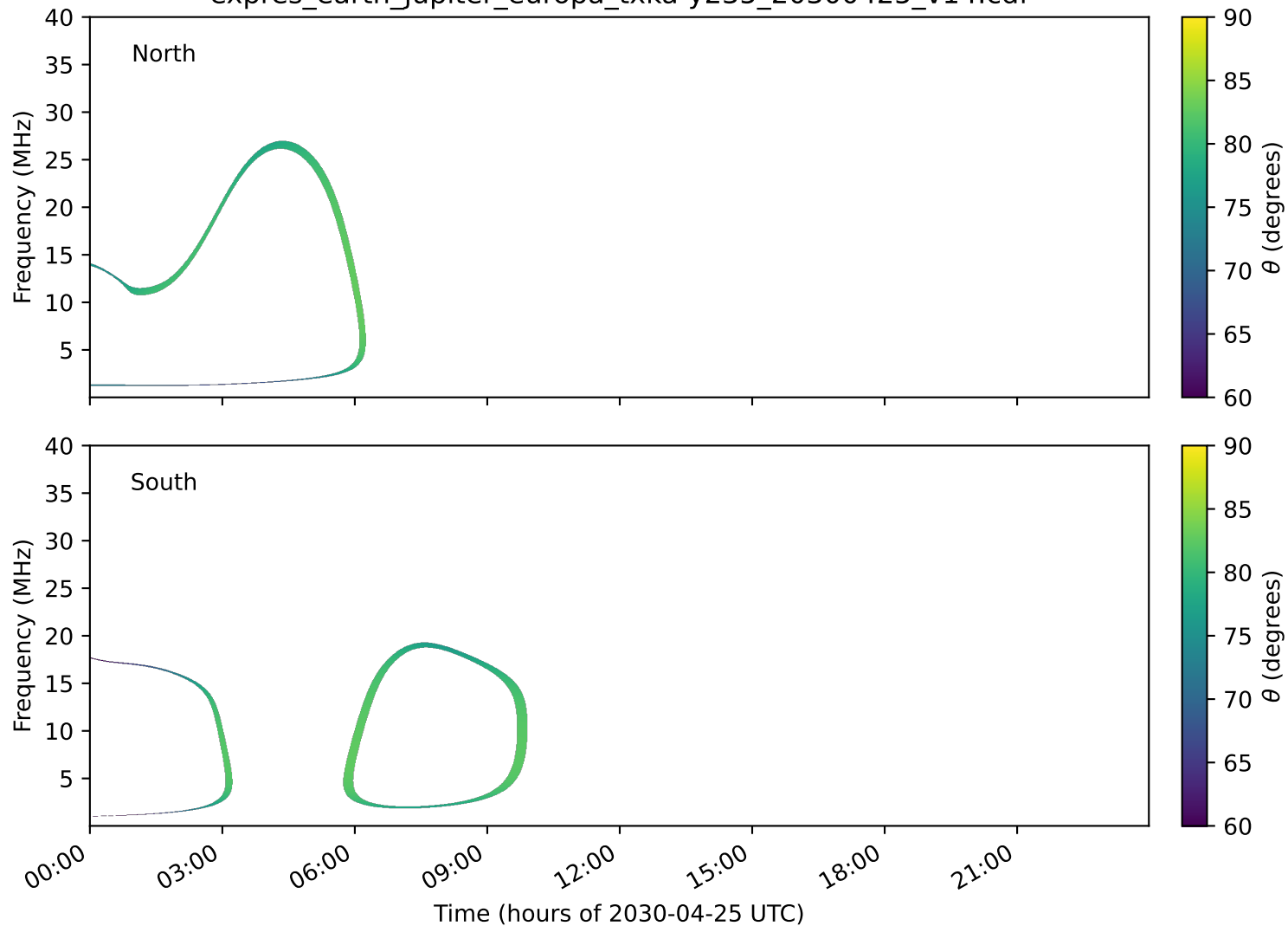
expres_earth_jupiter_europa_txka-y235_20300425_v14.cdf
