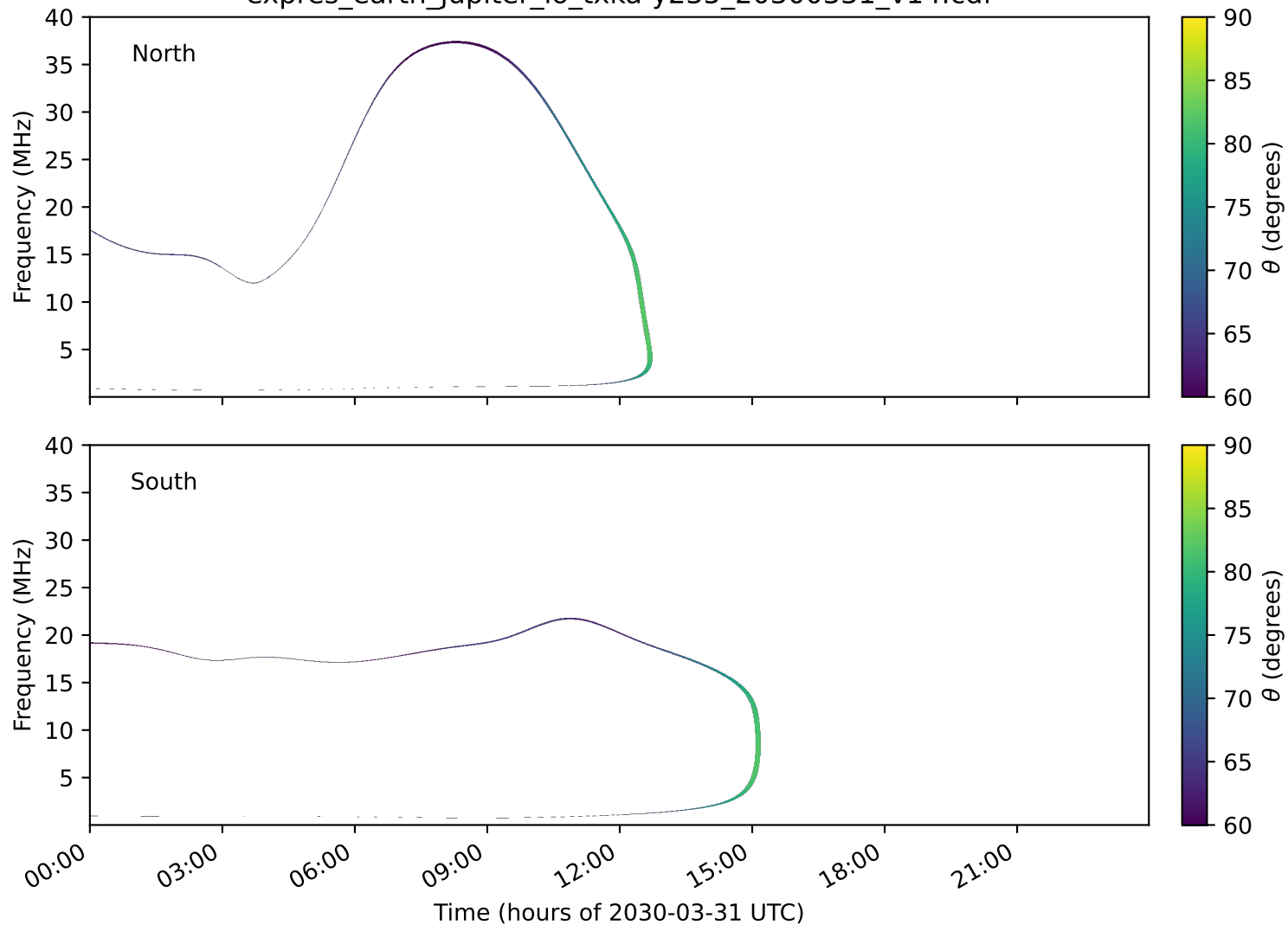
expres_earth_jupiter_io_txka-y235_20300331_v14.cdf
