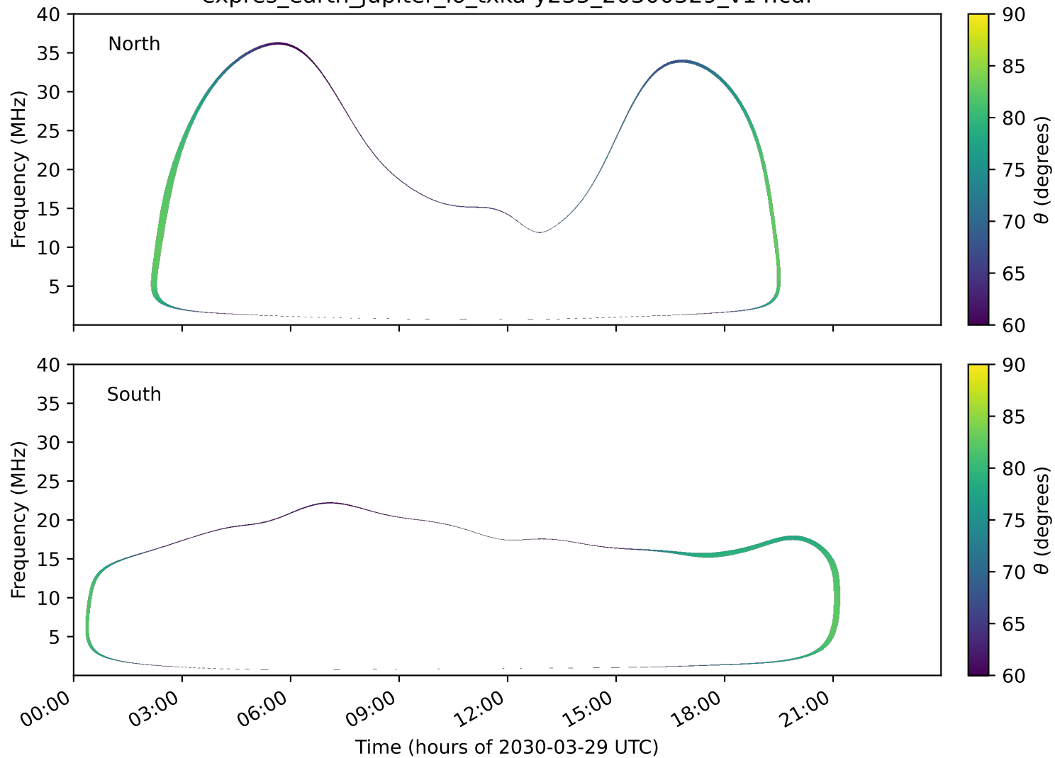
expres_earth_jupiter_io_txka-y235_20300329_v14.cdf
