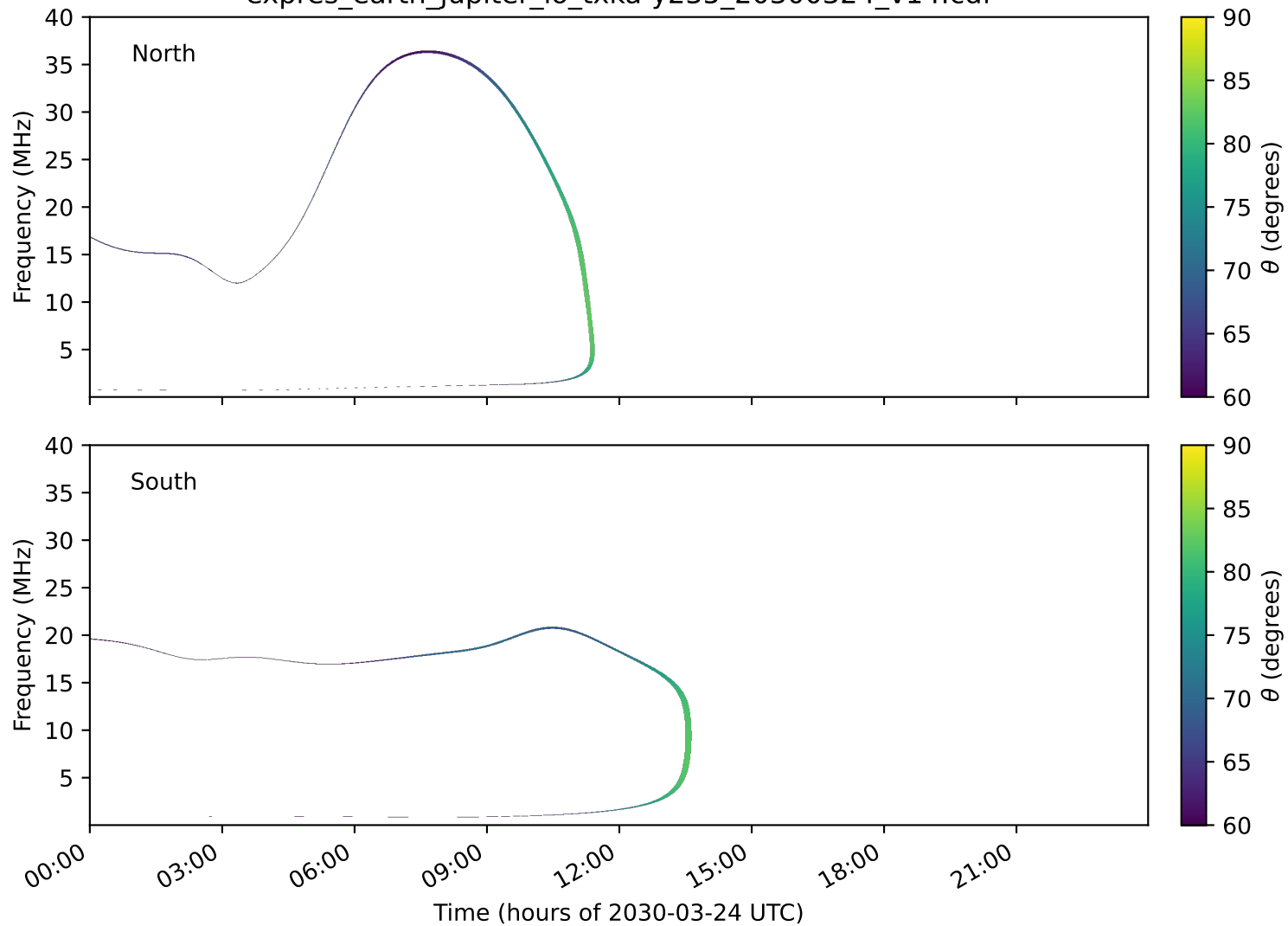
expres_earth_jupiter_io_txka-y235_20300324_v14.cdf
