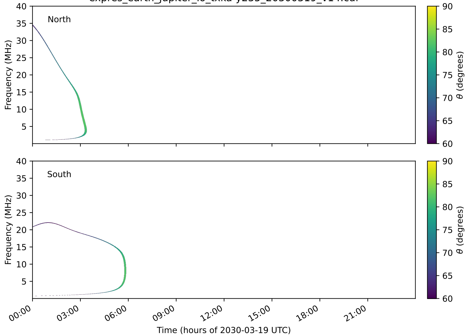
expres_earth_jupiter_io_txka-y235_20300319_v14.cdf
