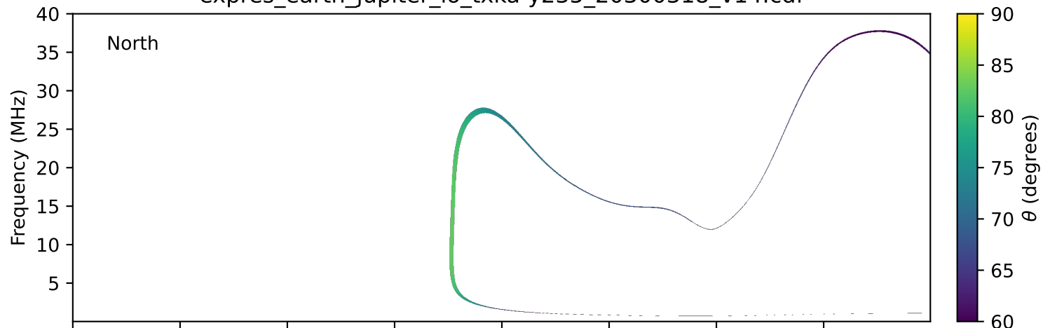
expres_earth_jupiter_io_txka-y235_20300318_v14.cdf
