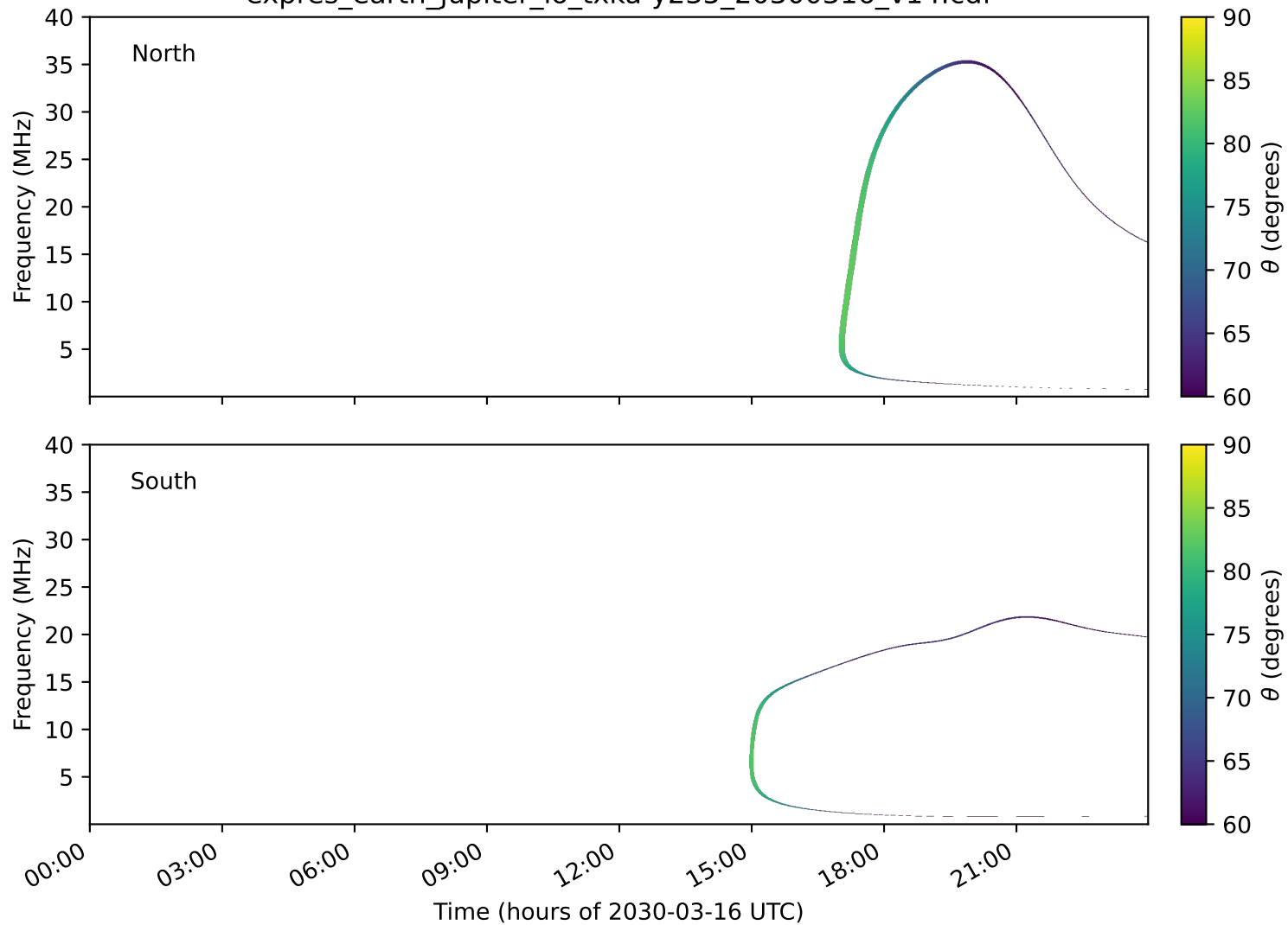
expres_earth_jupiter_io_txka-y235_20300316_v14.cdf
