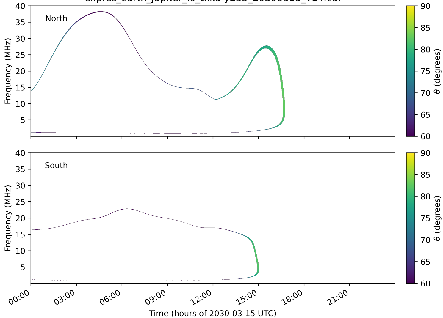
expres_earth_jupiter_io_txka-y235_20300315_v14.cdf
