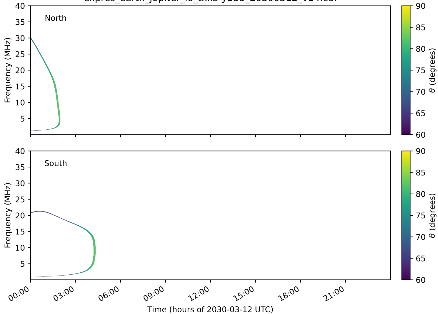
expres_earth_jupiter_io_txka-y235_20300312_v14.cdf
