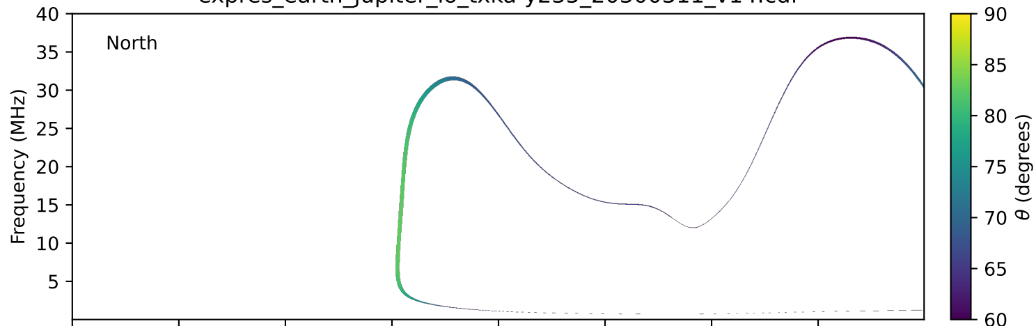
expres_earth_jupiter_io_txka-y235_20300311_v14.cdf
