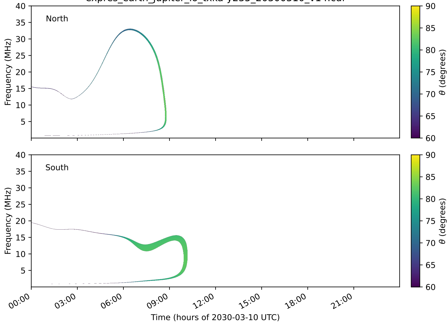
expres_earth_jupiter_io_txka-y235_20300310_v14.cdf
