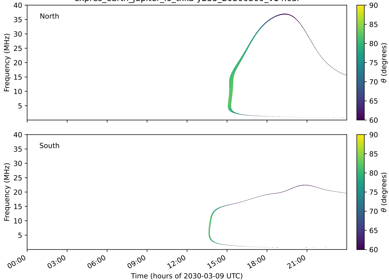
expres_earth_jupiter_io_txka-y235_20300309_v14.cdf
