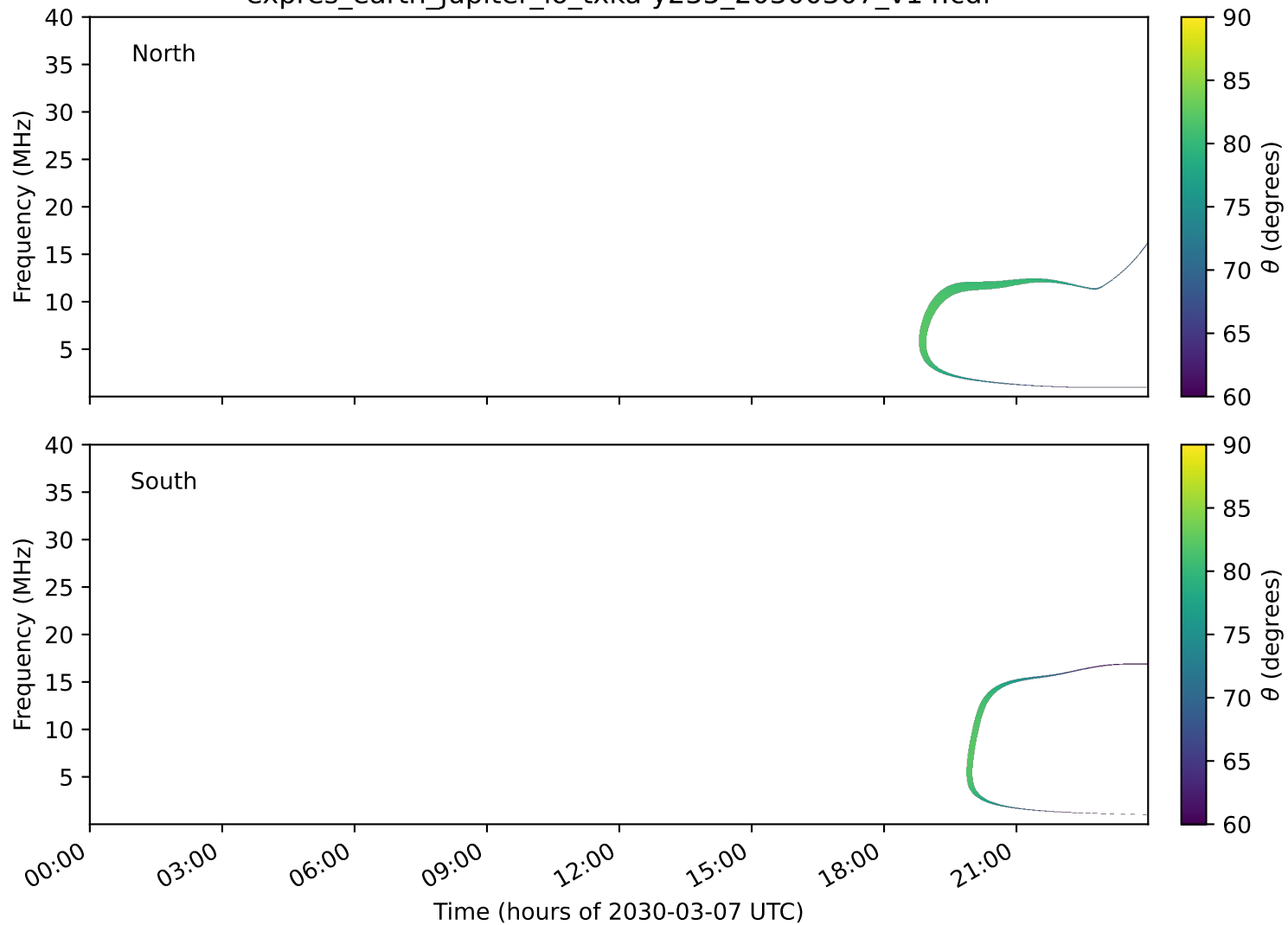
expres_earth_jupiter_io_txka-y235_20300307_v14.cdf
