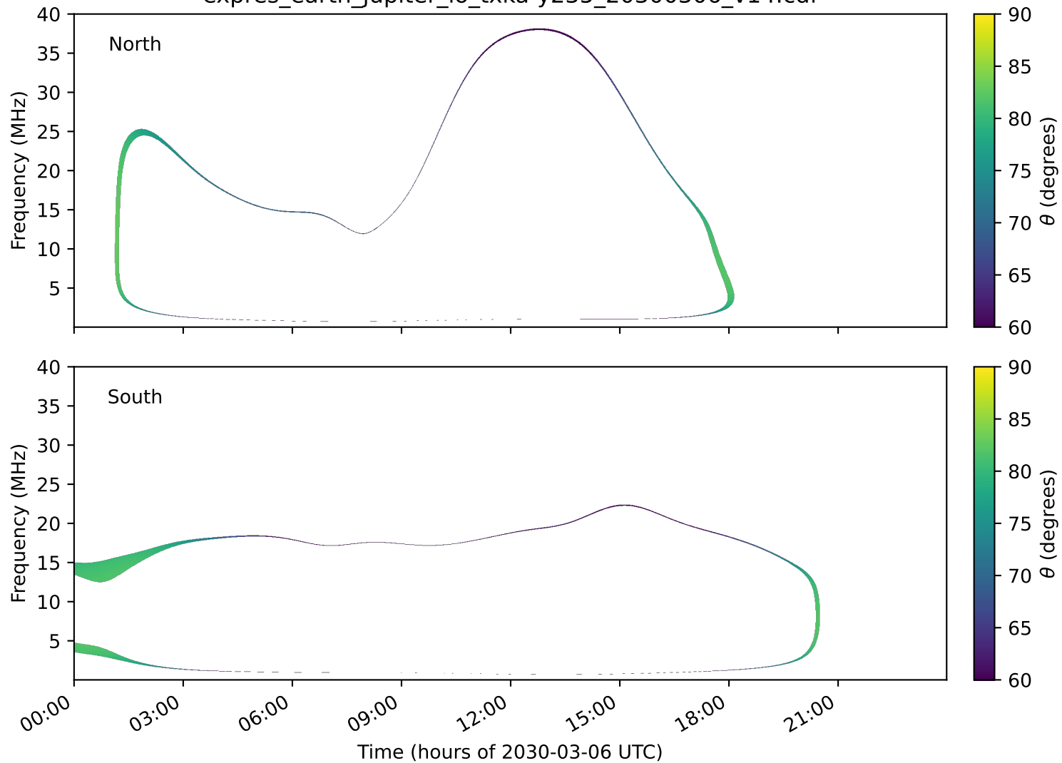
expres_earth_jupiter_io_txka-y235_20300306_v14.cdf
