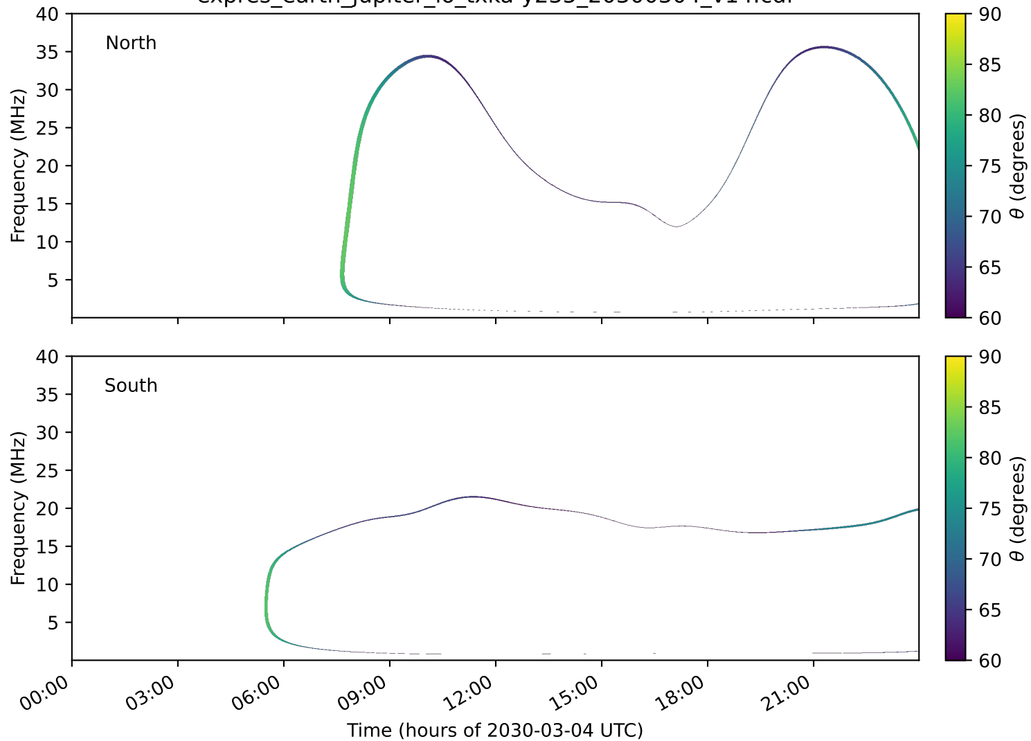
expres_earth_jupiter_io_txka-y235_20300304_v14.cdf
