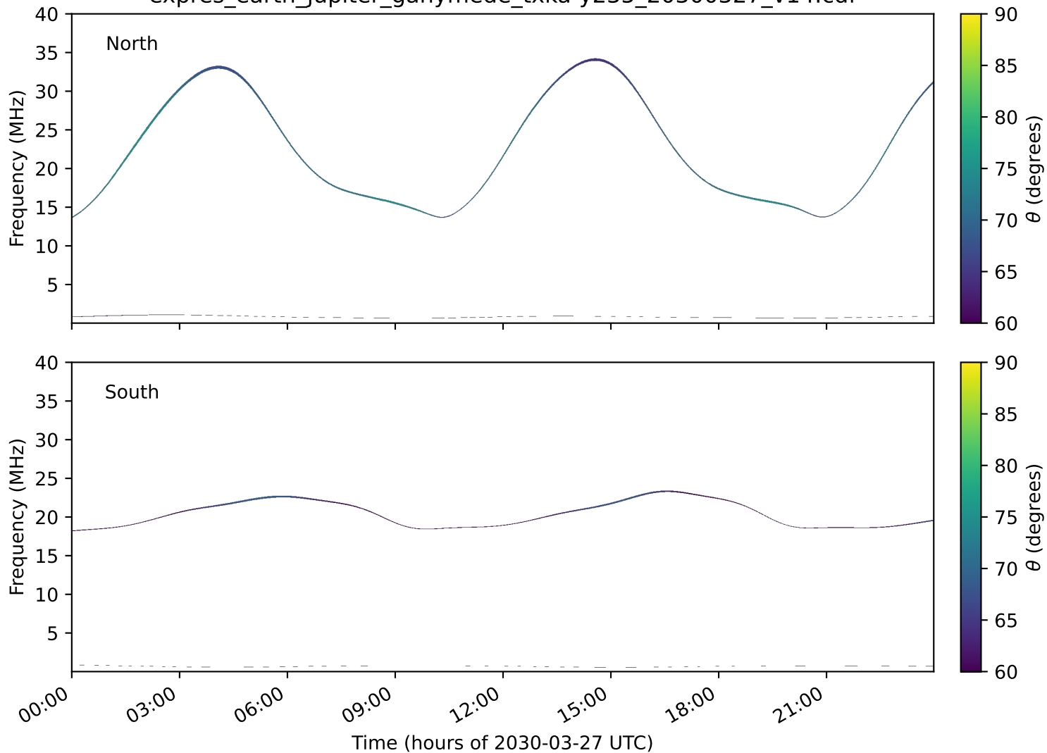
expres_earth_jupiter_ganymede_txka-y235_20300327_v14.cdf
