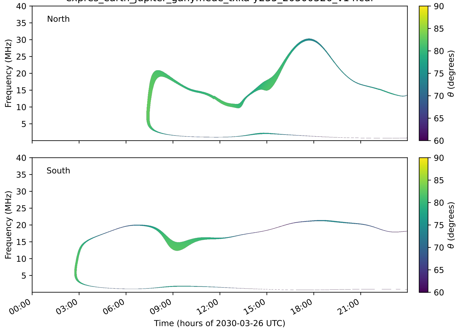
expres_earth_jupiter_ganymede_txka-y235_20300326_v14.cdf
