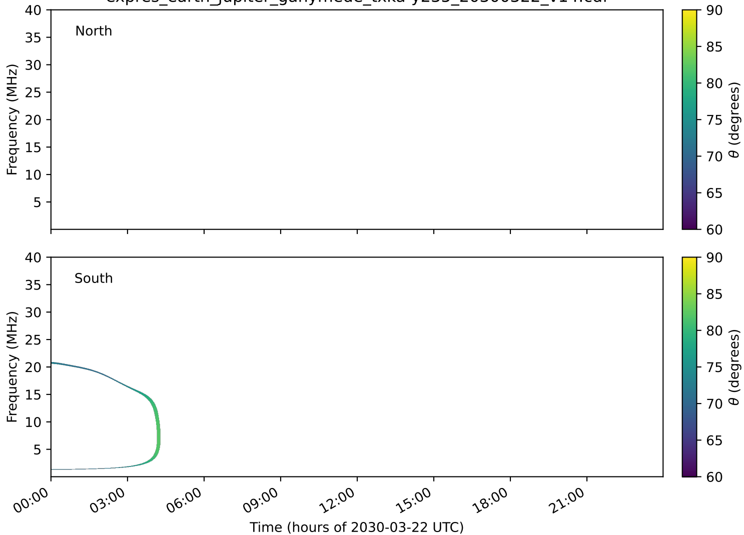
expres_earth_jupiter_ganymede_txka-y235_20300322_v14.cdf
