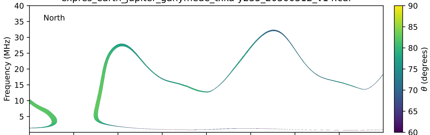
expres_earth_jupiter_ganymede_txka-y235_20300312_v14.cdf
