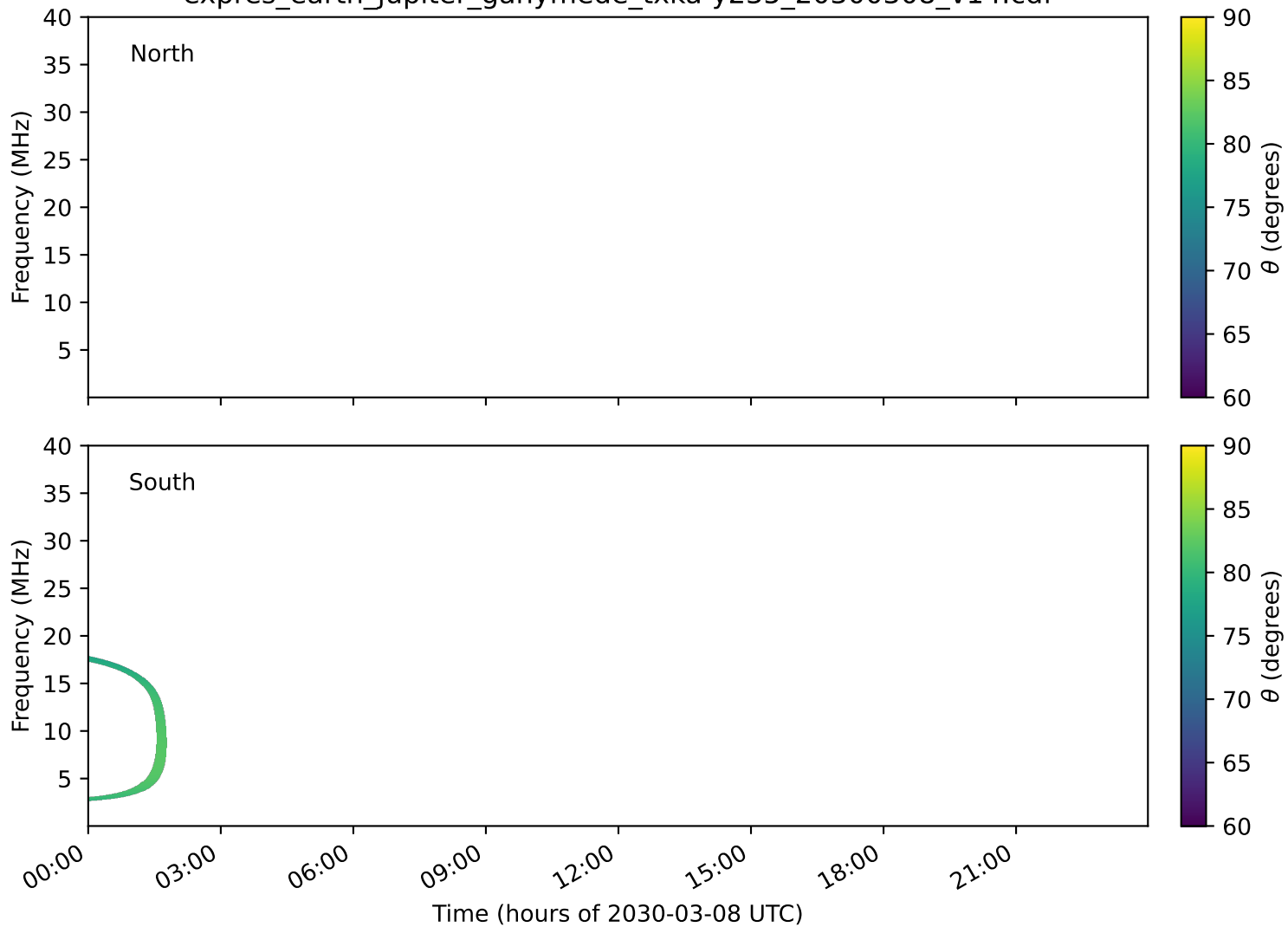
expres_earth_jupiter_ganymede_txka-y235_20300308_v14.cdf
