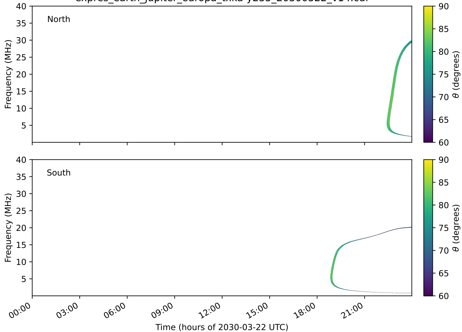
expres_earth_jupiter_europa_txka-y235_20300322_v14.cdf
