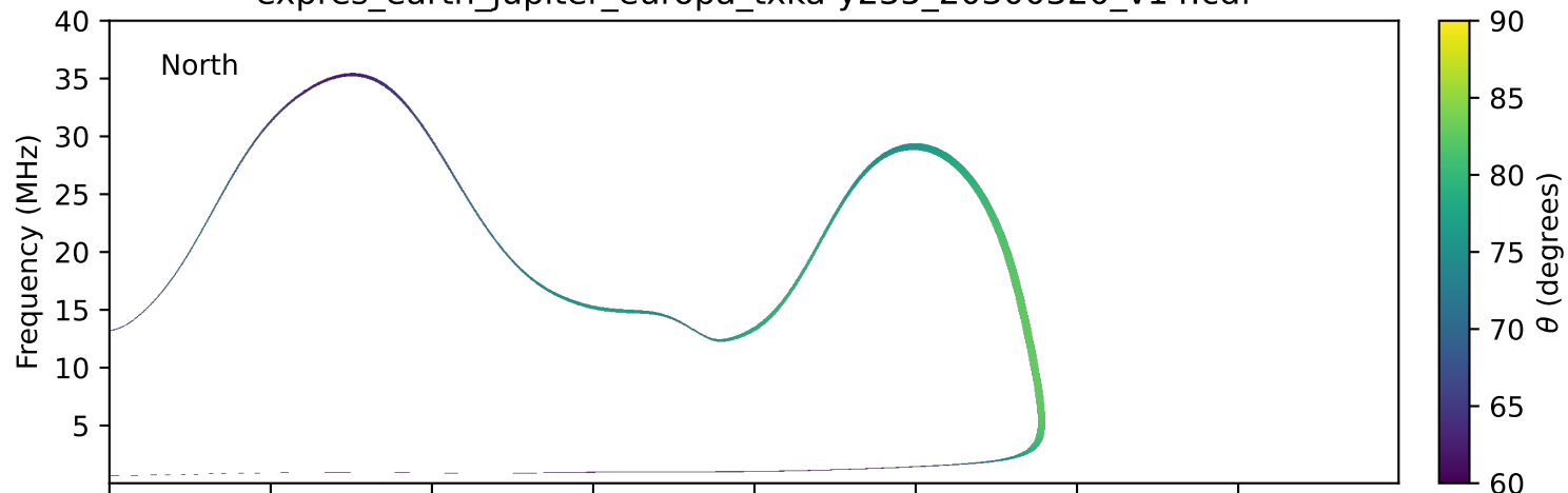
expres_earth_jupiter_europa_txka-y235_20300320_v14.cdf
