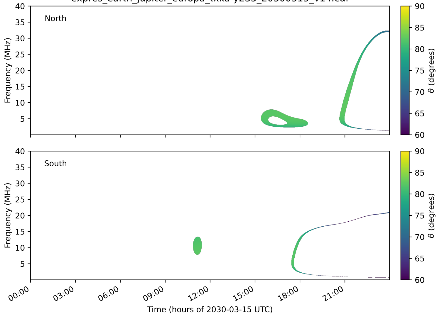
expres_earth_jupiter_europa_txka-y235_20300315_v14.cdf
