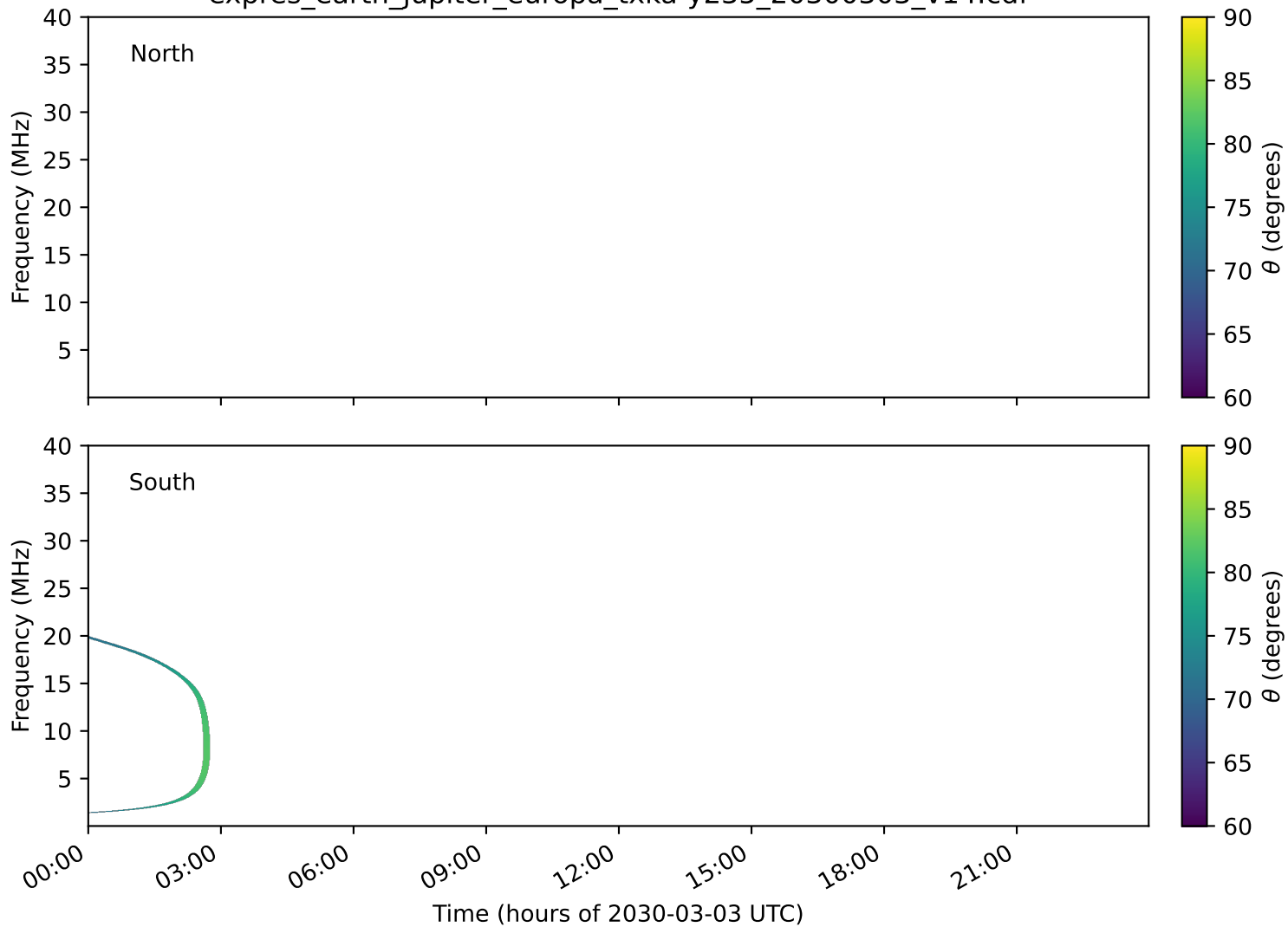
expres_earth_jupiter_europa_txka-y235_20300303_v14.cdf
