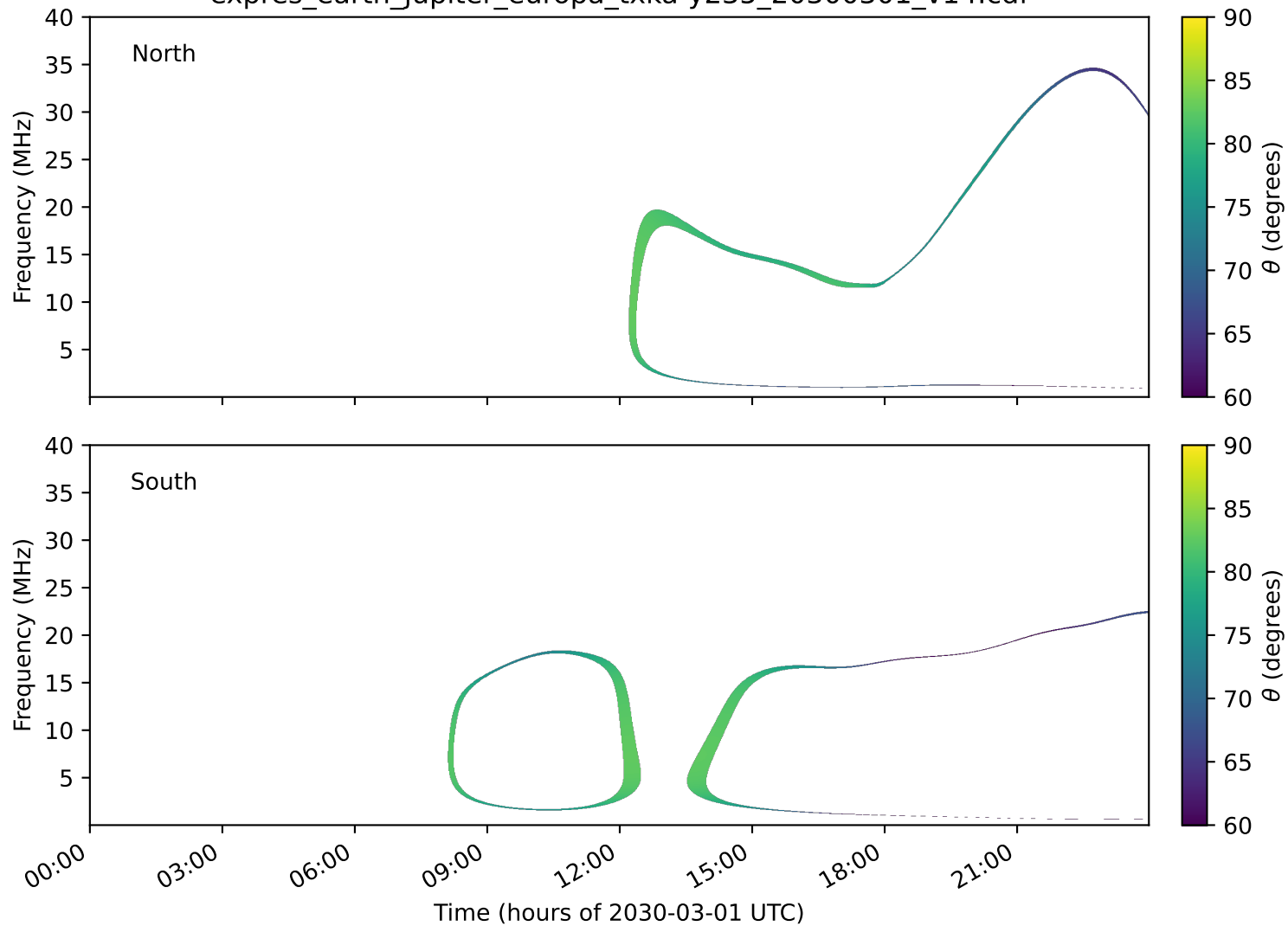
expres_earth_jupiter_europa_txka-y235_20300301_v14.cdf
