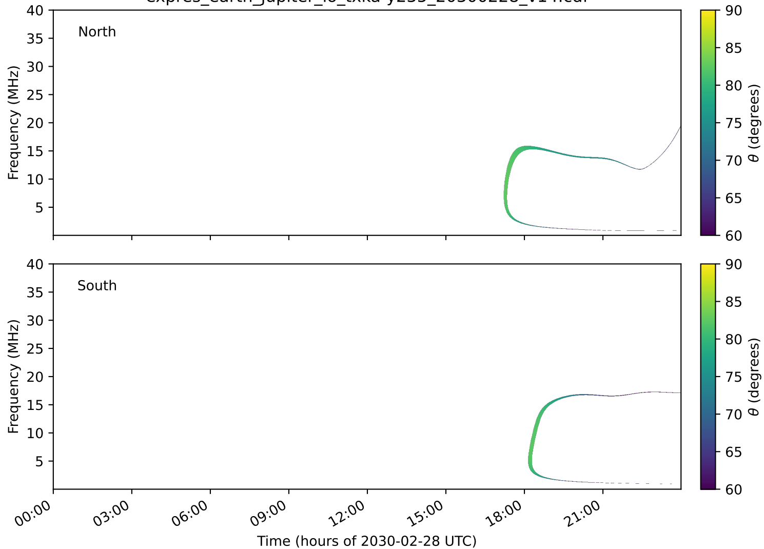
expres_earth_jupiter_io_txka-y235_20300228_v14.cdf
