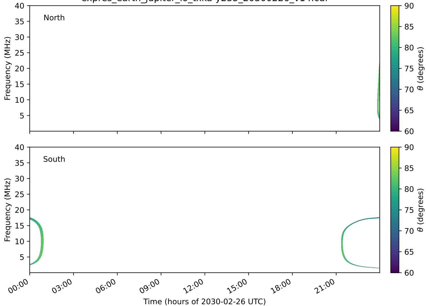
expres_earth_jupiter_io_txka-y235_20300226_v14.cdf
