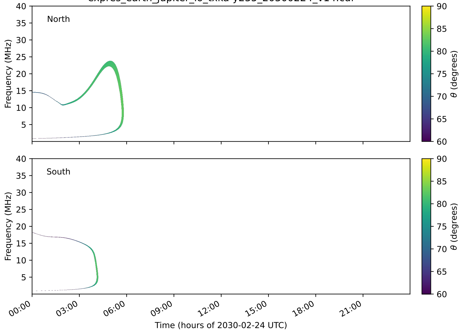
expres_earth_jupiter_io_txka-y235_20300224_v14.cdf
