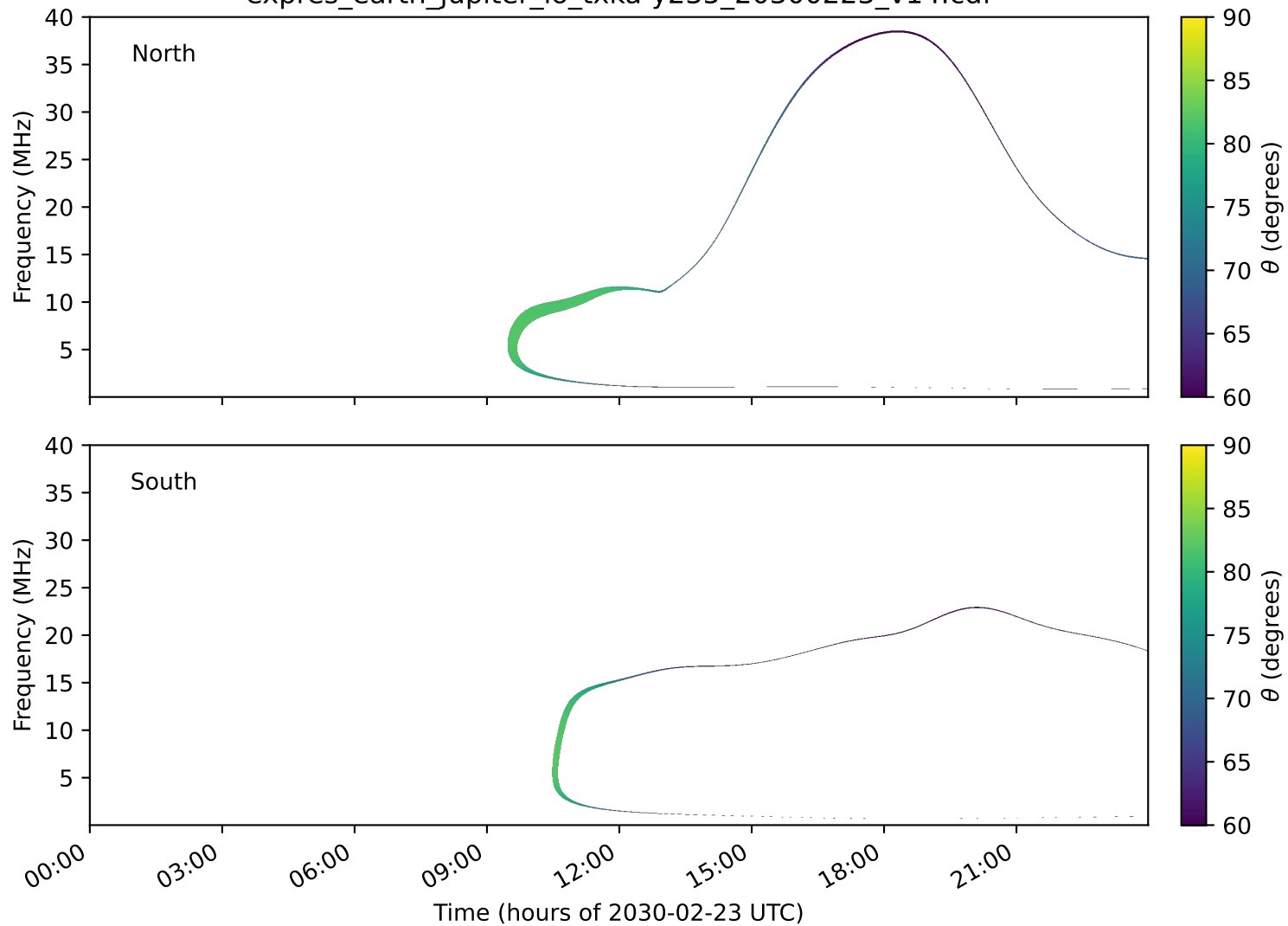
expres_earth_jupiter_io_txka-y235_20300223_v14.cdf
