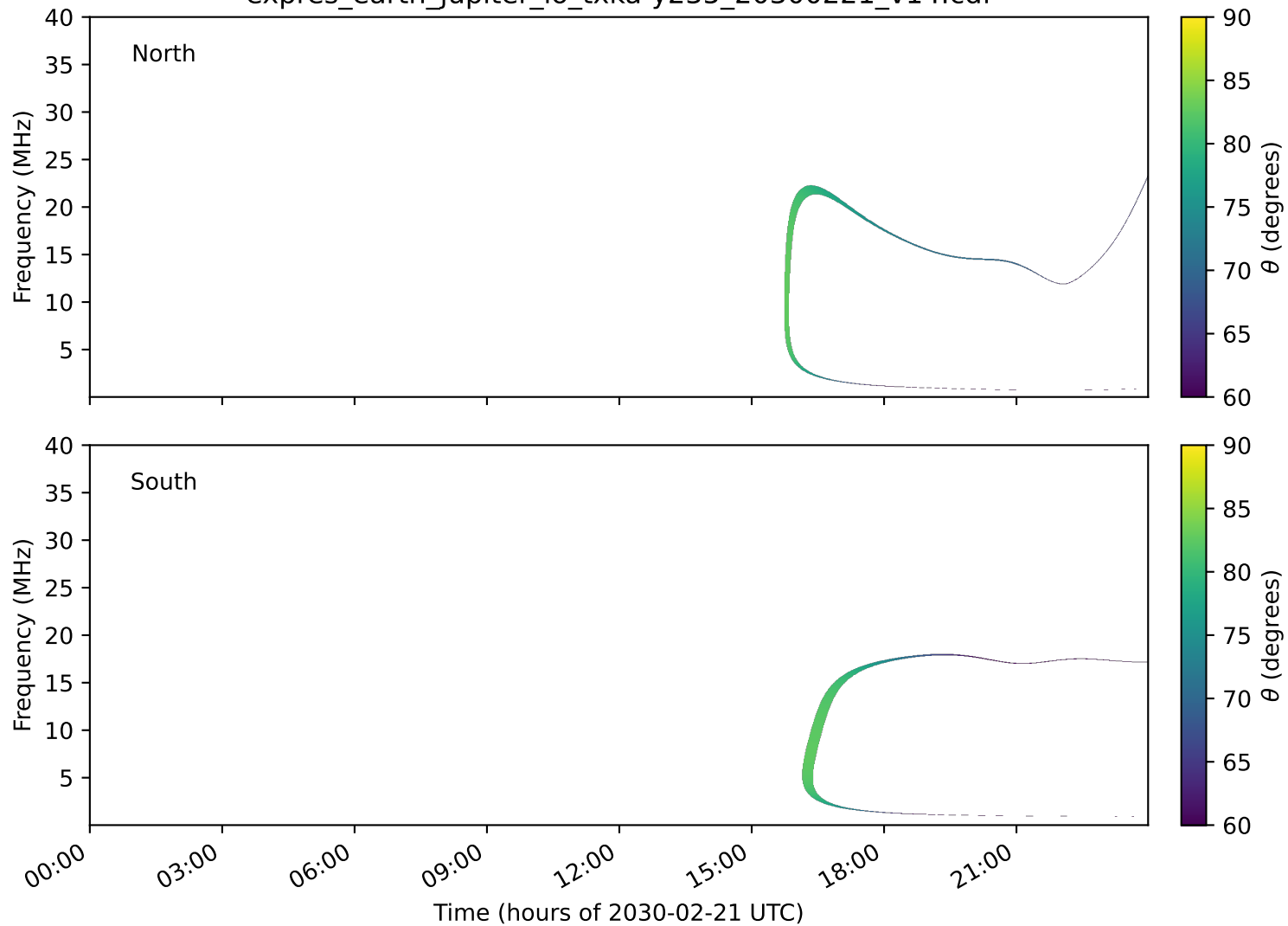
expres_earth_jupiter_io_txka-y235_20300221_v14.cdf
